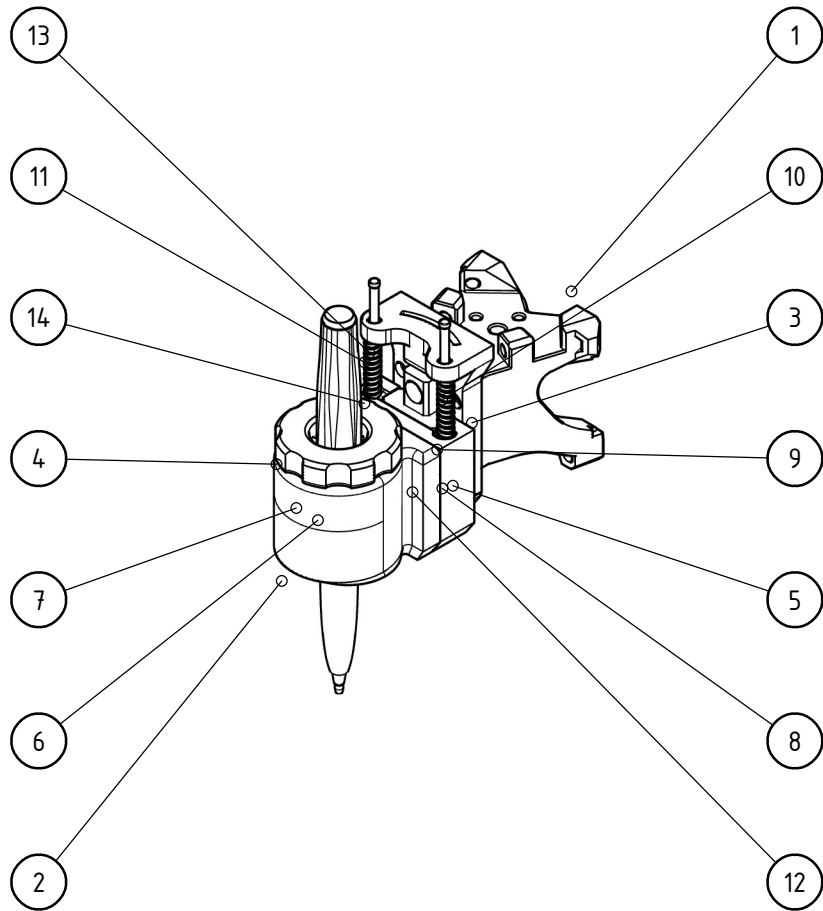
ISOMETRIC 1:2
