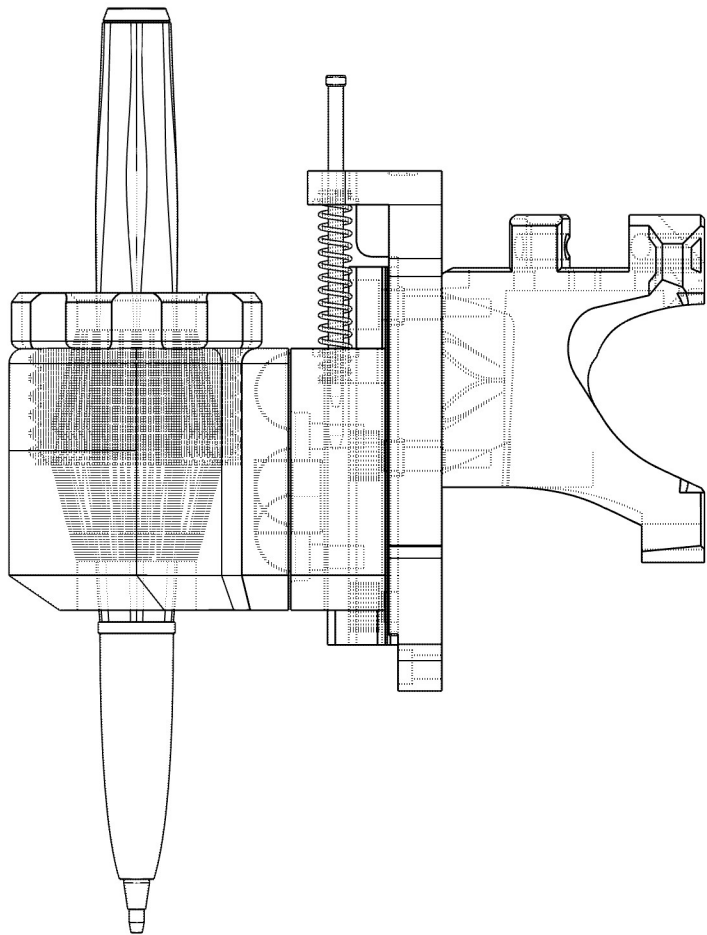
RIGHT SIDE
